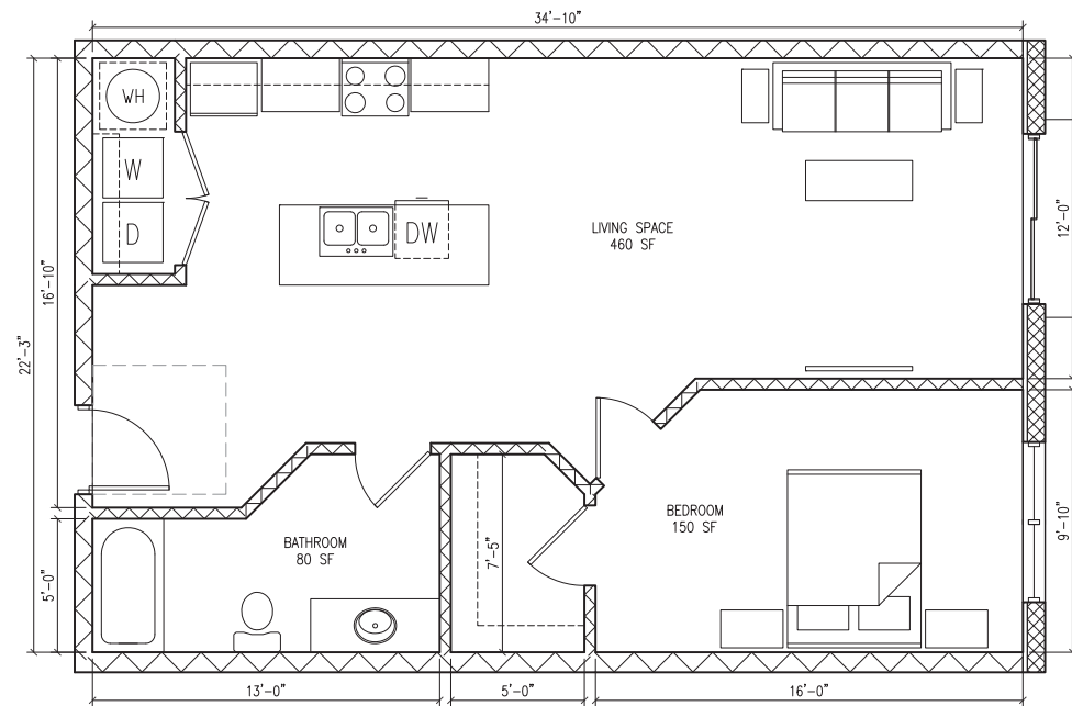
Unit C - 775 SF 1 bed / 1 bath
